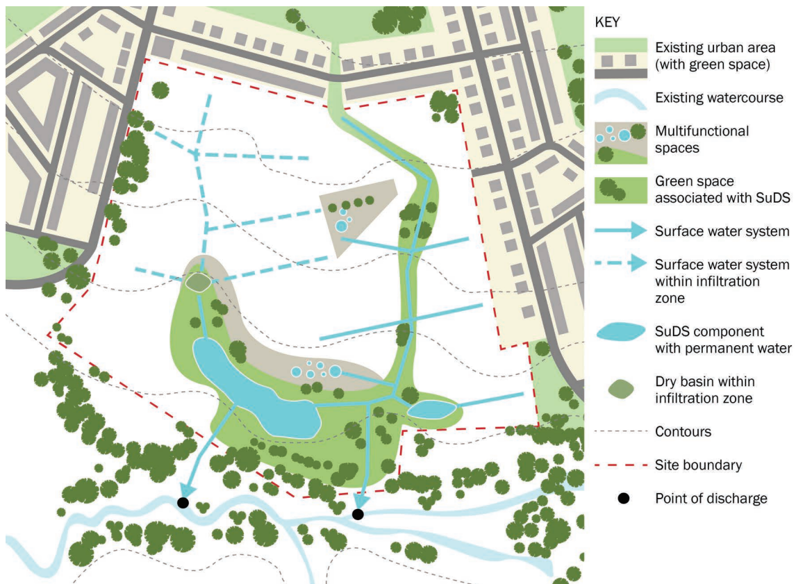
Figure 7.7 Defining parks, open spaces and corridors
