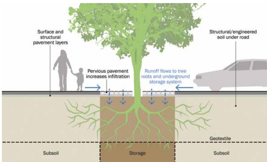
Figure 19.3 Collection of surface water runoff for trees
